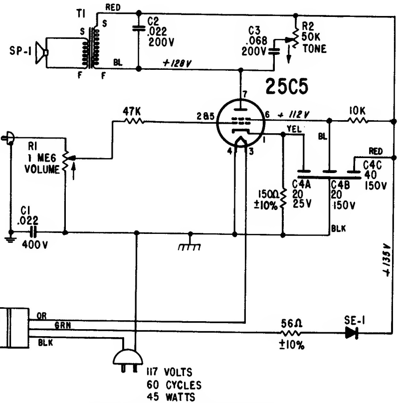
1L21 SCHEMATIC FOR MODEL LP8.
